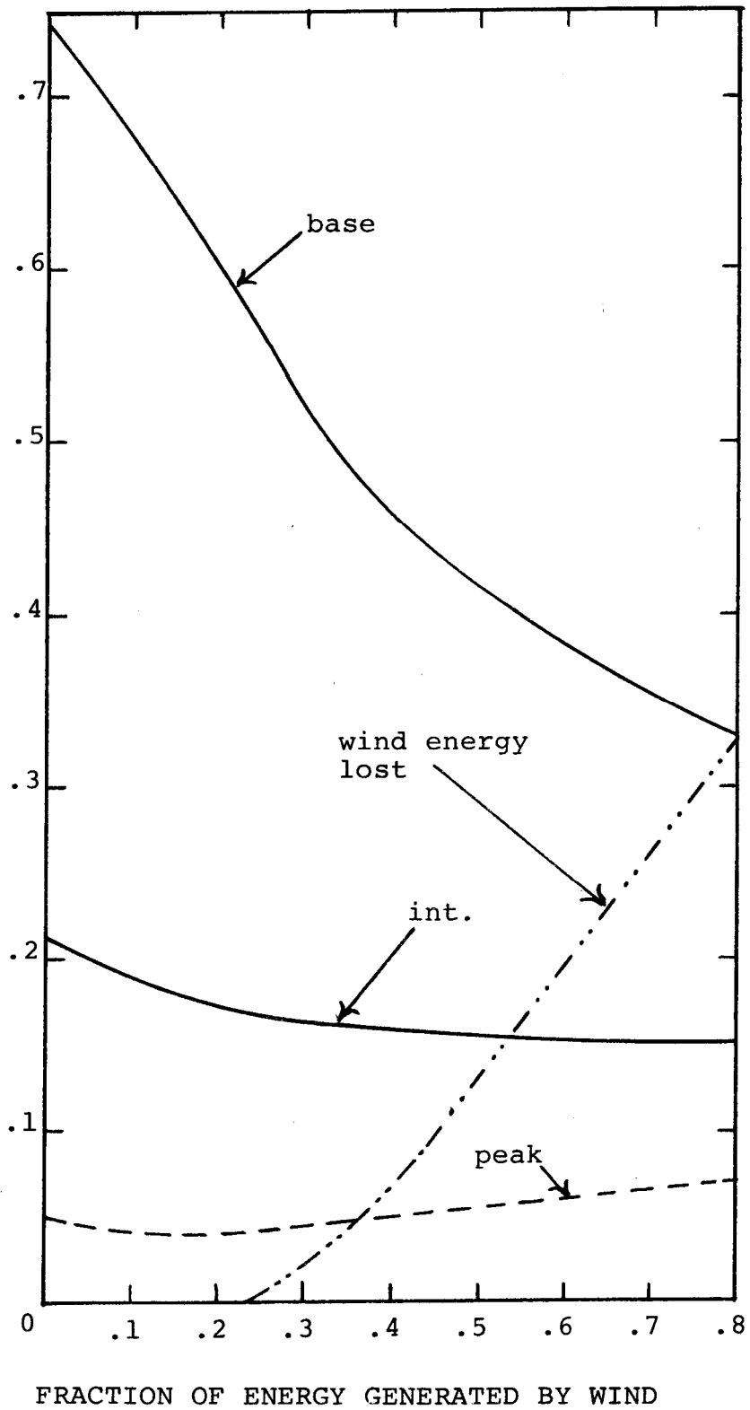
Figure 4 Reduction in the consumption of natural gas and coal, and the increase in lost (wind) energy, as a function of wind energy input to the 1978 SA grid, approximate model. ( \alpha = 1 and v_T/\bar{v} = 1.5 ). Base plant burn gas, intermediate burn coal
